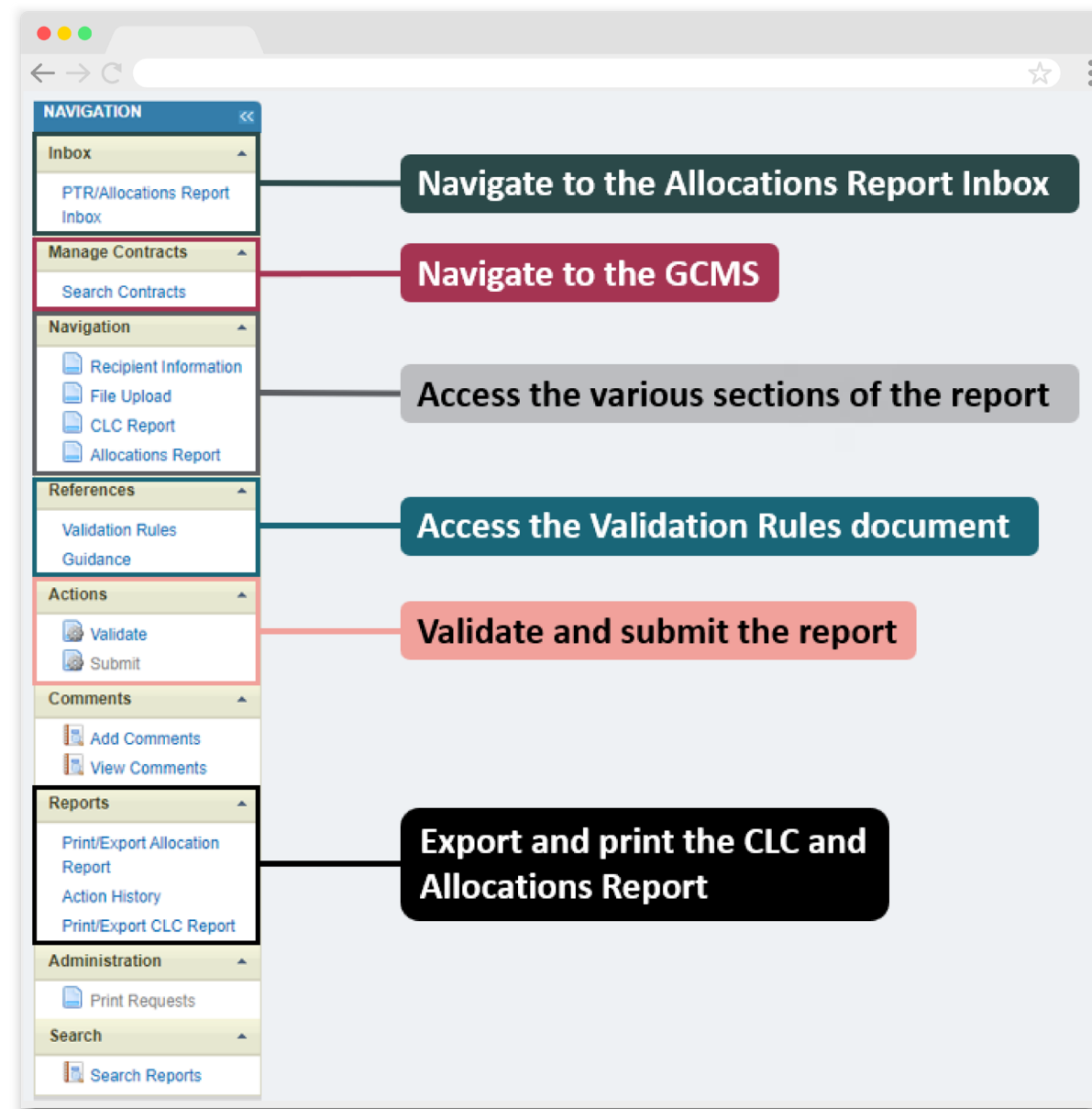
Figure 5. Allocations Report Navigation Panel Guide
